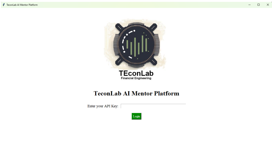
Image 1. Login Screen
